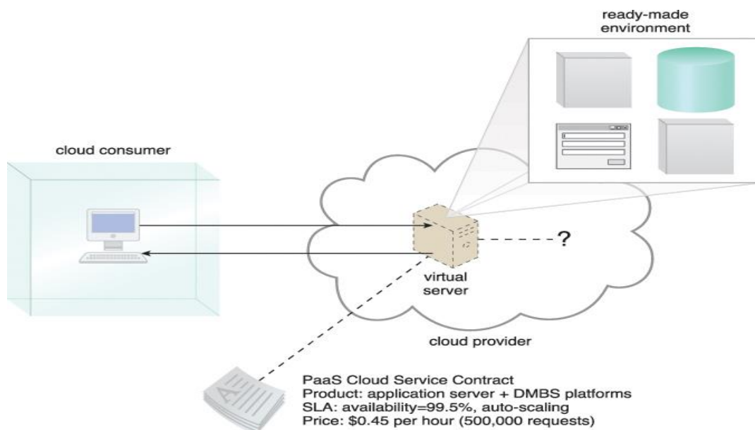
Fig 2.1: PaaS
