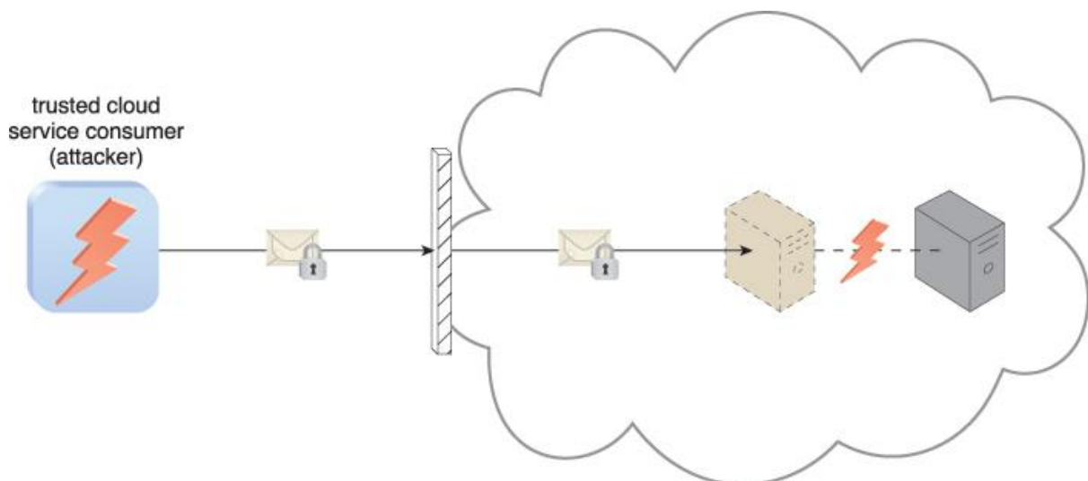
Fig 4.3: Virtualization attack
