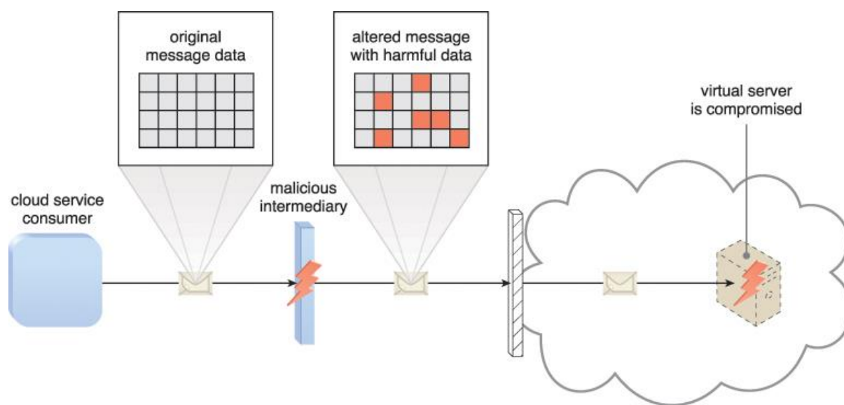
Fig 4.4: Malicious intermediary
