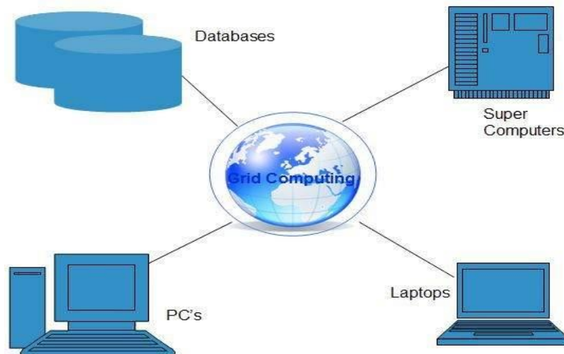
Figure 1.2: Grid Computing
