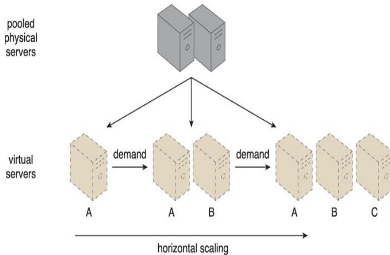
Figure 1.6: Horizontal scaling
