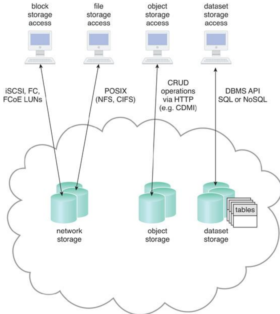
Fig 5.4: Cloud storage
