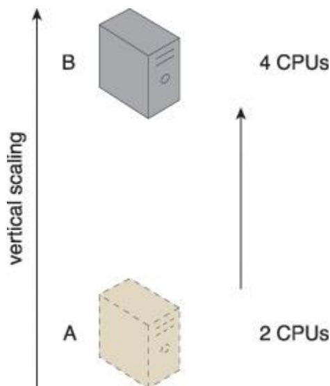
Figure 1.7 : Vertical scaling
